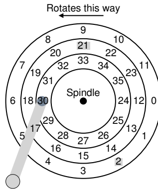
Figure 37.7: SSTF: Scheduling Requests 21 And 2
